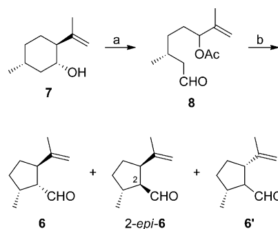
Scheme 2. Enantioselective preparation of (–)-photocitral A ( 6 ) from (–)-isopulegol ( 7 ). a) Pb(OAc) 4 , CaCO 3 , benzene, reflux, 74%; b) 5 mol% [Pd(PPh 3 ) 4 ], 40 mol% pyrrolidine, Et 3 N, THF, –10°C, 89% ( 6 /2- epi - 6 / 6' = 47:43:10).
