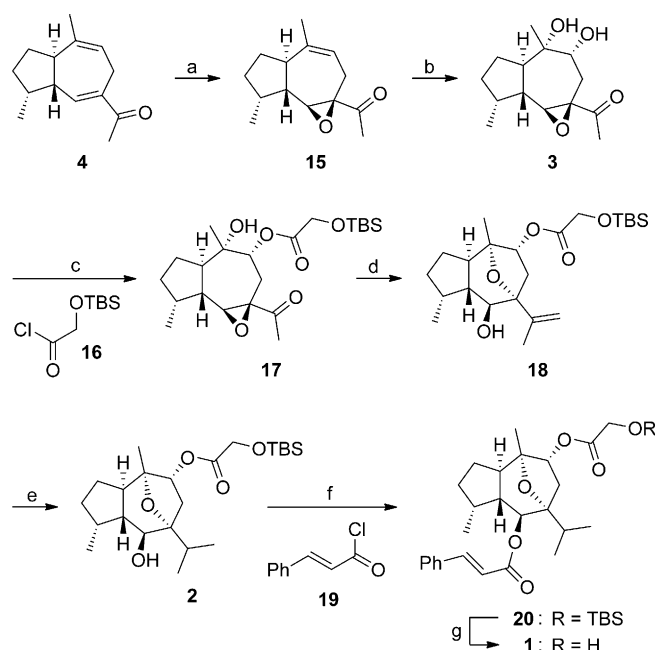
Scheme 4. Completion of the synthesis. a) \text{NaOH} , \text{H}_2\text{O}_2 , \text{MeOH} , RT, 91%; b) 1 mol % \text{K}_2\text{OsO}_4 , NMO, acetone, water, THF, RT, 97%, d.r. = 2:1; c) 16 , pyridine, RT, 93%; d) \text{Ph}_3\text{P}=\text{CH}_2 , THF, RT, then 2 N \text{HCl} , 70%; e) 1 atm \text{H}_2 , 10% \text{Pd/C(en)} , \text{EtOH} , RT, 90%; f) 19 , DMAP, \text{Et}_3\text{N} , \text{CH}_2\text{Cl}_2 , reflux, 94%; g) 2 N \text{HCl} , THF, RT, 100%. NMO = N -methylmorpholin- N -oxide, en = ethylenediamine, DMAP = 4-(dimethylamino)pyridine.
