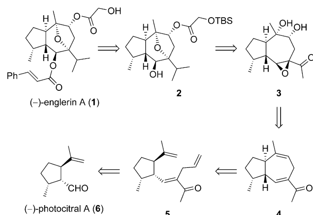
Scheme 1. Retrosynthetic tracing of (–)-englerin A ( 1 ) to (–)-photocitral A ( 6 ). TBS = tert -butyldimethylsilyl.
