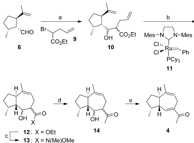
Scheme 3. Construction of the hydroazulene framework. a) 9 , Zn, benzene, reflux, 86%; b) 1 mol % 11 , \text{CH}_2\text{Cl}_2 , reflux, 99%; c) \text{MeONH-Me-HCl} , i\text{PrMgCl} , THF, -30^\circ\text{C} \rightarrow \text{reflux} ; d) \text{MeLi} , THF, -78^\circ\text{C} \rightarrow \text{RT} , 73% (2 steps); e) 1. \text{MsCl} , \text{Et}_3\text{N} , \text{CH}_2\text{Cl}_2 , 0^\circ\text{C} ; 2. DBU, RT, 85% (94% based on recovered 14 ). Ms = methanesulfonyl, DBU = 1,8-diazabicyclo[5.4.0]undec-7-ene.
